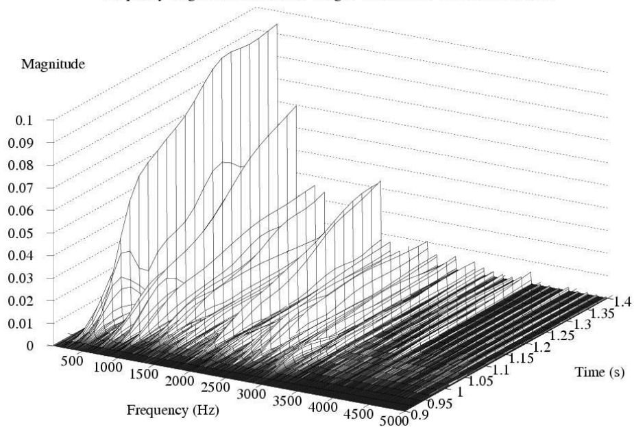
Spec3dw plot 18-09-2007 10:21:17, file: a20070912-saksalainen.raw, sampling rate: 44100Hz, FFT points: 8192, window length: 8192, type: hanning, increment: 1000, frequency range: 100-5000Hz, HF weight: 1, comment: Saksalainen, c-kieli
