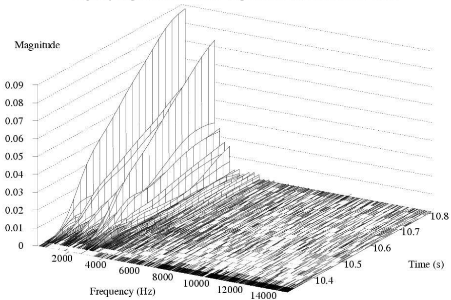
Spec3dw plot 18-09-2007 10:56:43, file: a20070912-saksalainen.raw, sampling rate: 44100Hz, FFT points: 8192, window length: 8192, type: hanning, increment: 1000, frequency range: 100-15000Hz, HF weight: 1, comment: Saksalainen, d-kieli
