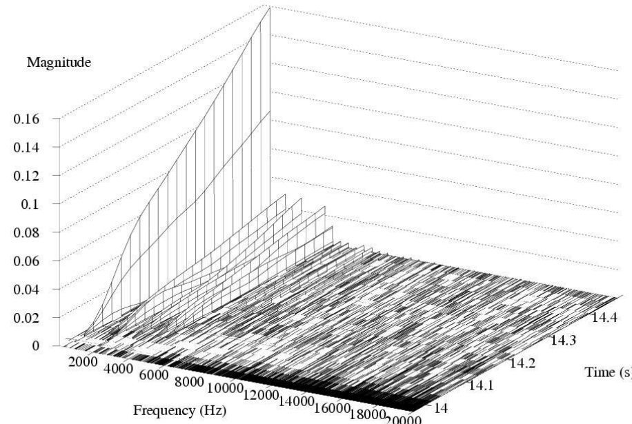
Spec3dw plot 18-09-2007 11:16:13, file: a20070912-saksalainen.raw, sampling rate: 44100Hz, FFT points: 8192, window length: 8192, type: hanning, increment: 1000, frequency range: 100-20000Hz, HF weight: 1, comment: Saksalainen, a-kieli
