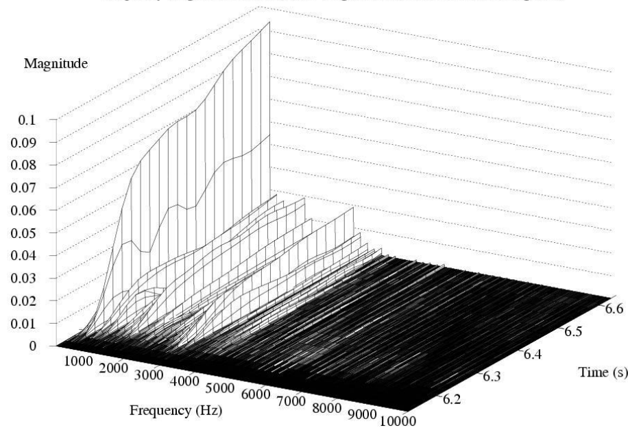
Spec3dw plot 18-09-2007 10:31:30, file: a20070912-saksalainen.raw, sampling rate: 44100Hz, FFT points: 8192, window length: 8192, type: hanning, increment: 1000, frequency range: 100-10000Hz, HF weight: 1, comment: Saksalainen, g-kieli
